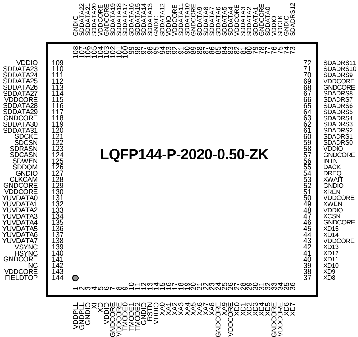
Figure 2 144-Pin LQFP Pin Configuration
